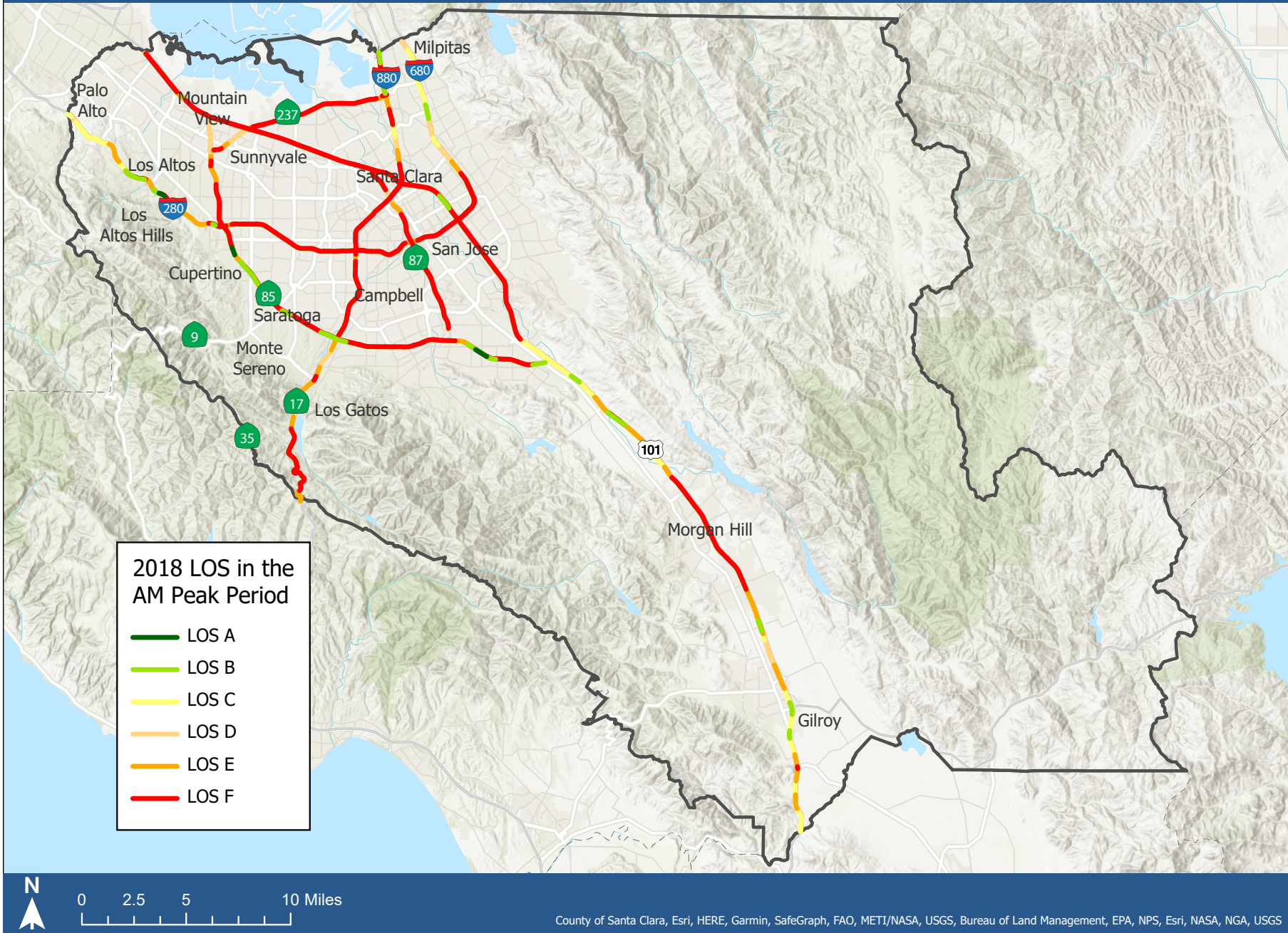
Figure 3.5 | 2018 Freeway Mixed Flow Level of Service in the AM Peak Period
